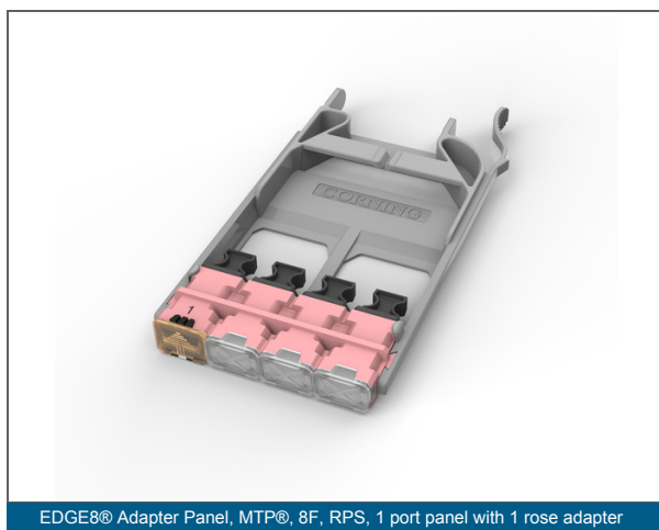
EDGE8® Adapter Panel, MTP®, 8F, RPS, 1 port panel with 1 rose adapter
